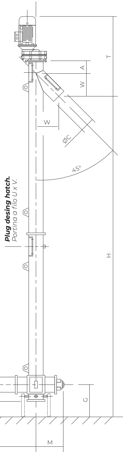
VERTICAL SCREW CONVEYORS CVS TYPE – COCLEE VERTICALI SERIE CVS – DIM (mm)
