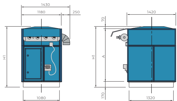
Assembly EKO BO model without electric fan
