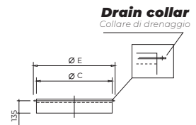
Filter mounting upstand Anello sottofiltro a saldare
